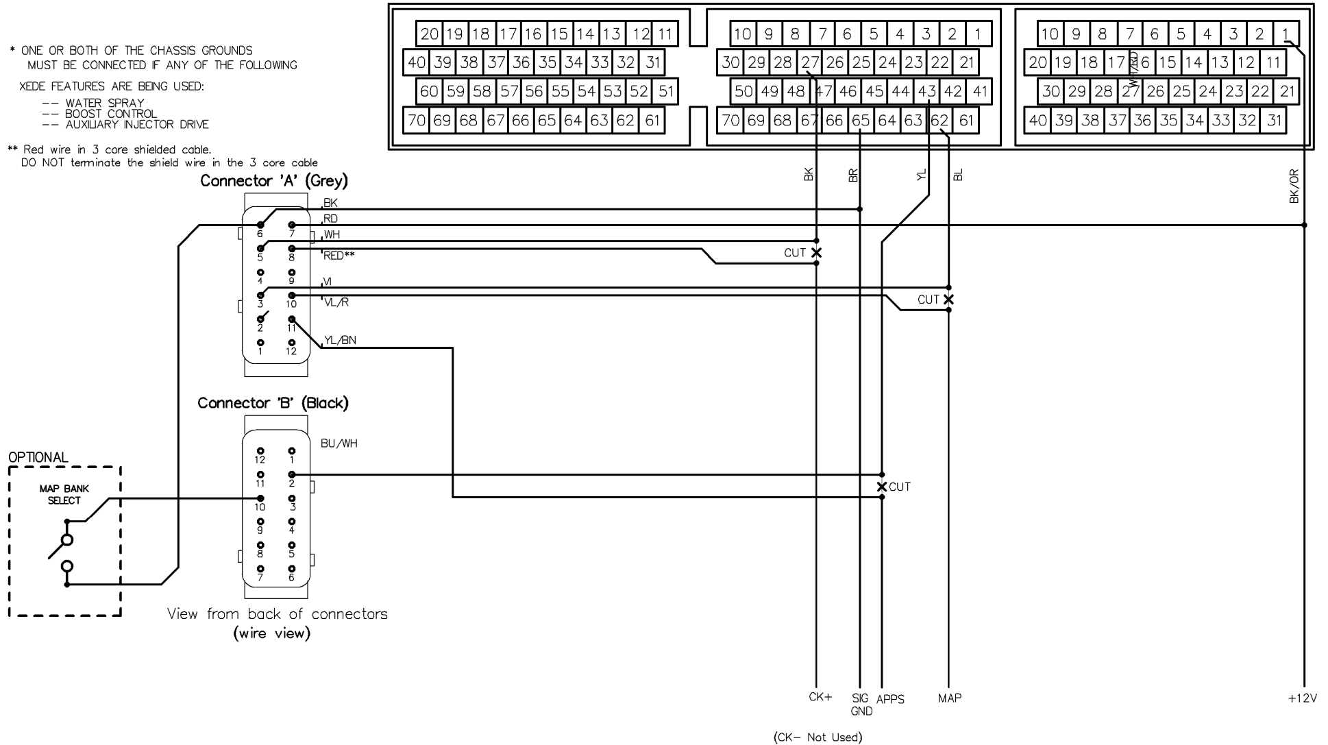
ECU View from back of connectors (wire view)
